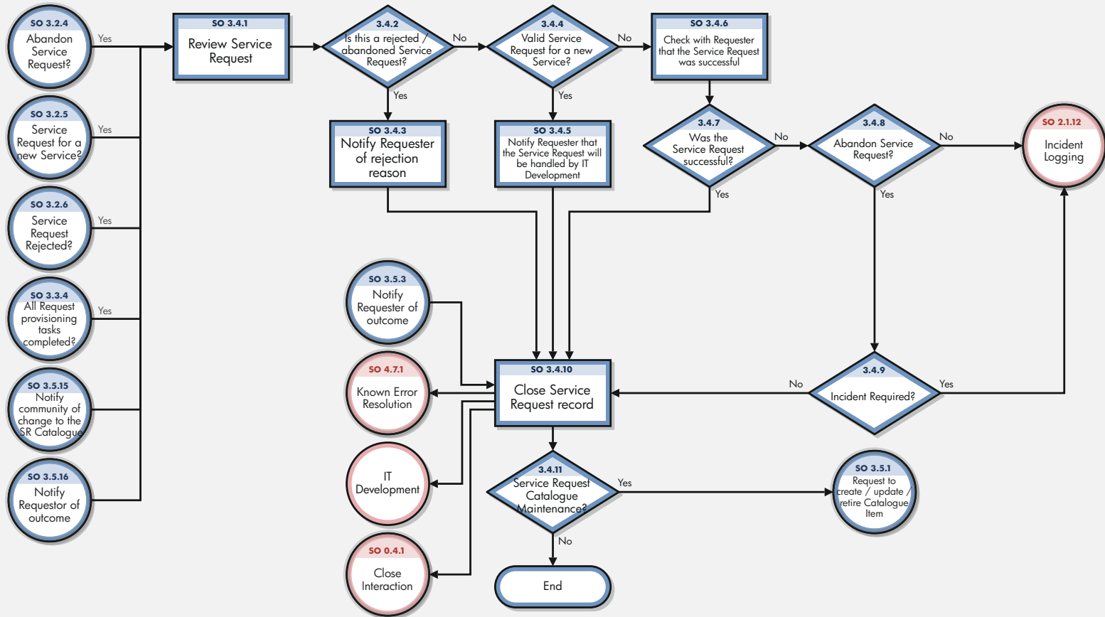
Figure 9-4 Service Request Validation and Closure workflow
