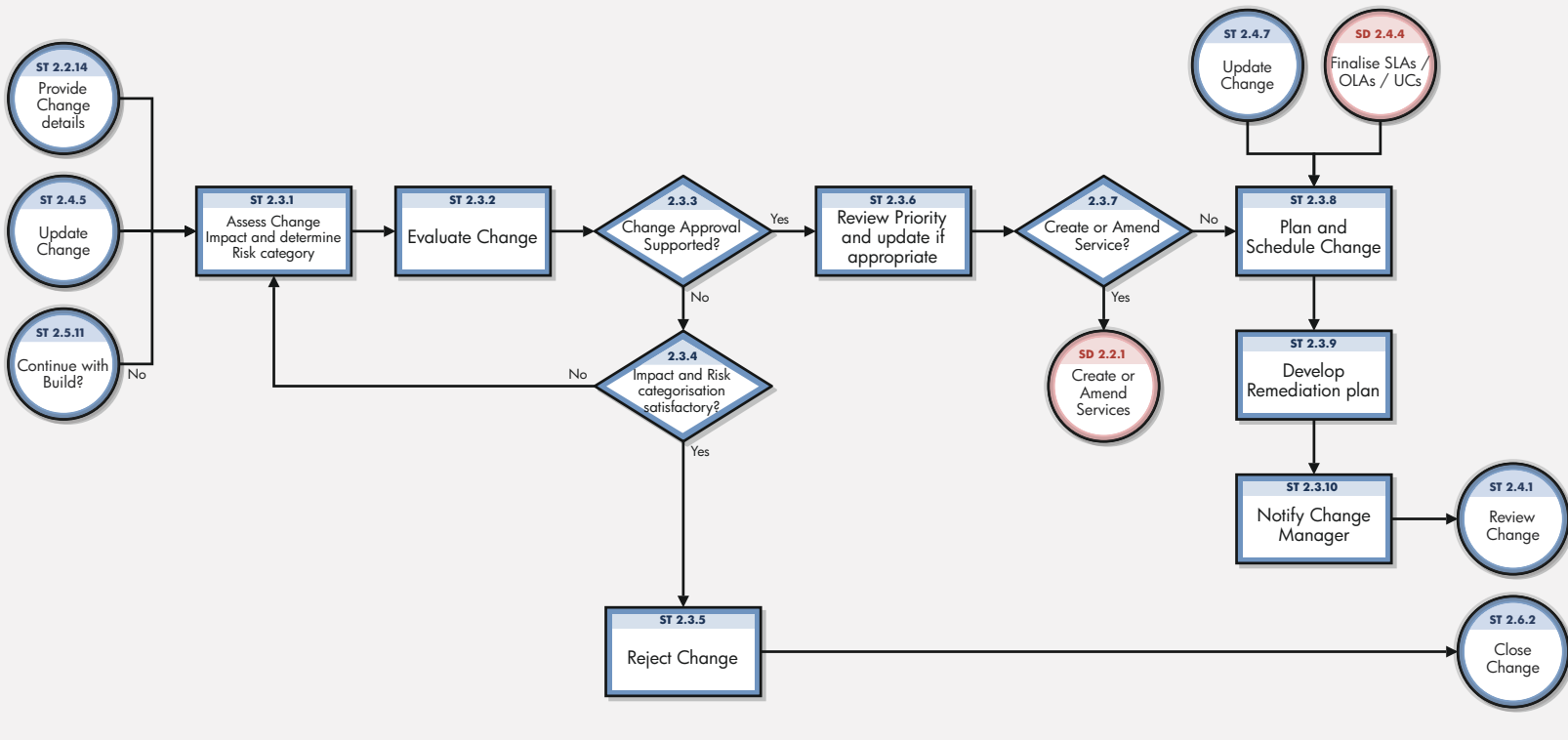
Figure 15-3 Change Assessment and Planning workflow
